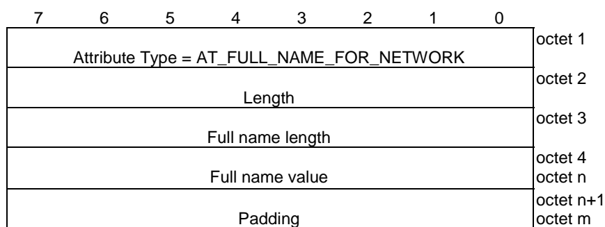
Figure 8.2.5.1-1: AT_FULL_NAME_FOR_NETWORK attribute
