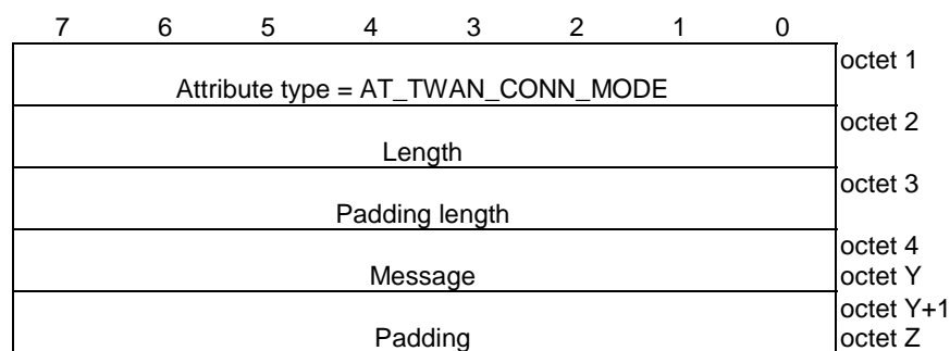
Figure 8.2.7.1-1: AT_TWAN_CONN_MODE attribute
