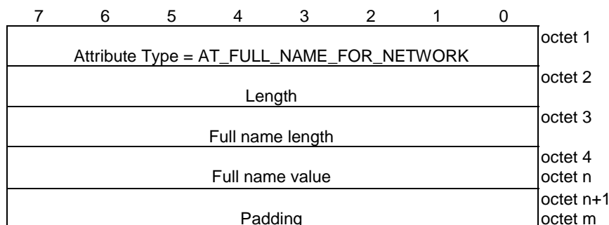
Figure 8.2.5.1-1: AT_FULL_NAME_FOR_NETWORK attribute
