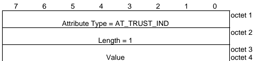
Figure 8.2.3.1-1: AT_TRUST_IND attribute
