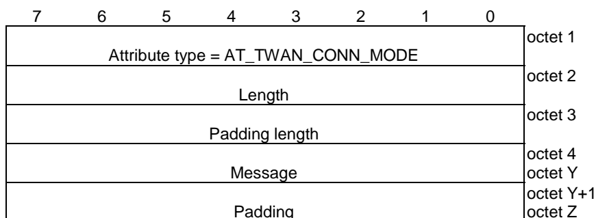
Figure 8.2.7.1-1: AT_TWAN_CONN_MODE attribute
