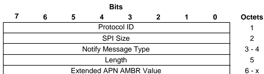
Figure 8.2.9.14-1: EXTENDED_APN_AMBR Notify payload format
