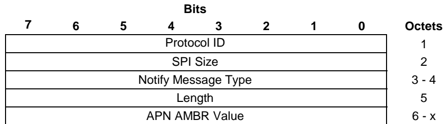
Figure 8.2.9.13-1: APN_AMBR Notify payload format
