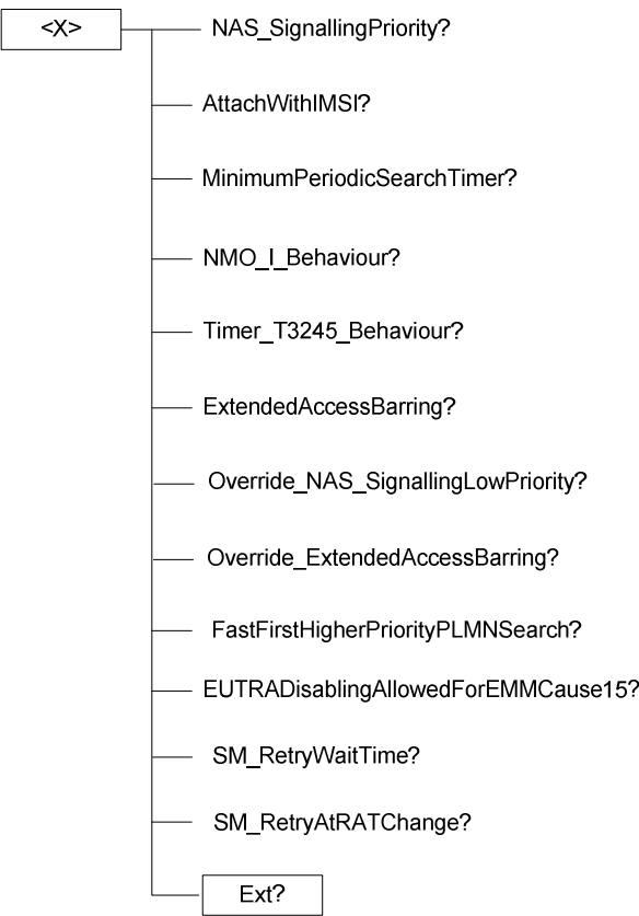
Figure 4-1: The NAS configuration Management Object
