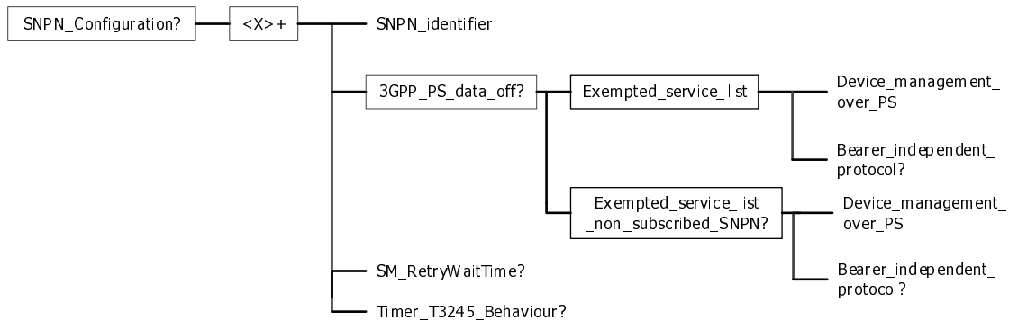
Figure 4-3: The NAS configuration Management Object (3 of 3)
