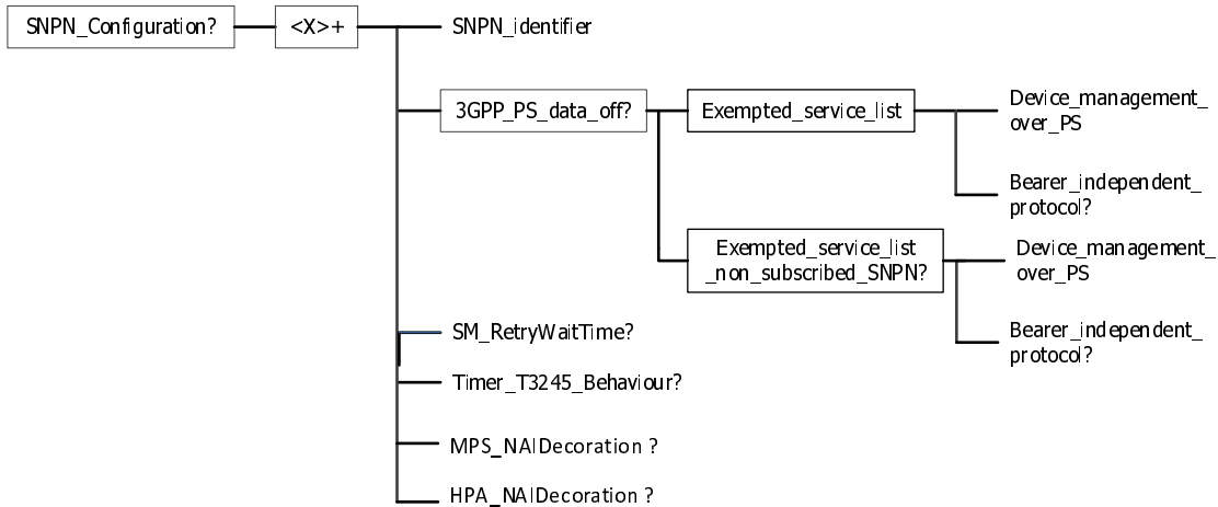
Figure 4-2: The NAS configuration Management Object (2 of 4)
