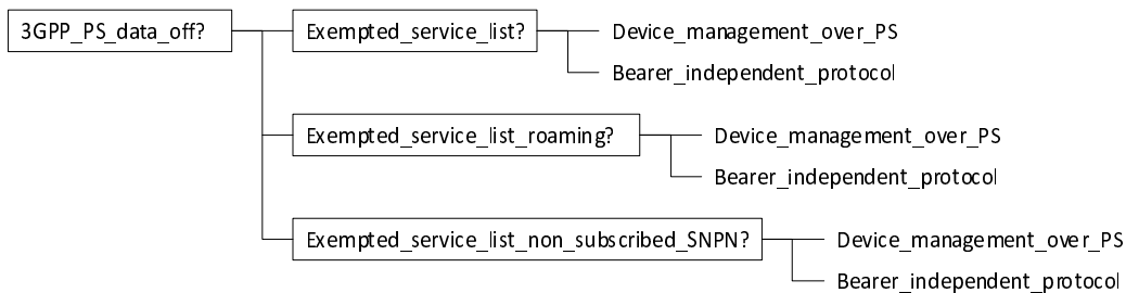
Figure 4-4: The NAS configuration Management Object (4 of 4)
