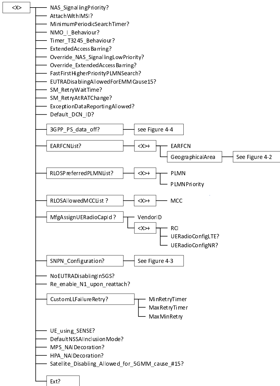
Figure 4-1: The NAS configuration Management Object (1 of 4)
