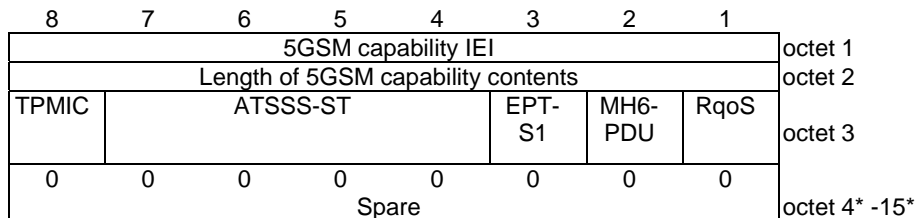
Figure 9.11.4.1.1: 5GSM capability information element
