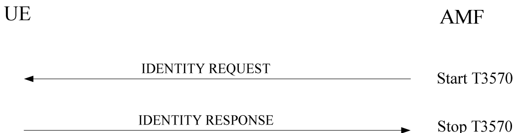
Figure 5.4.3.2.1: Identification procedure
