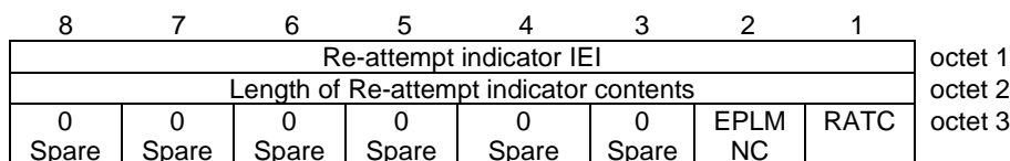
Figure 9.11.4.17.1: Re-attempt indicator
