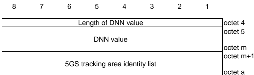
Figure 9.11.3.30.2: LADN
