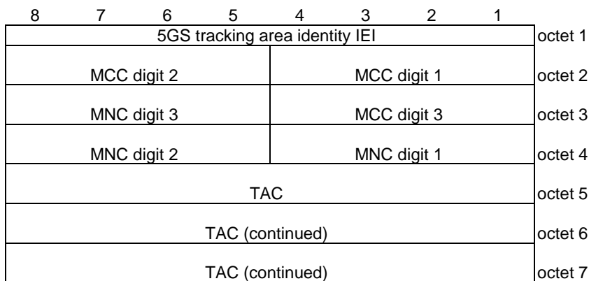
Figure 9.11.3.8.1: 5GS tracking area identity information element
