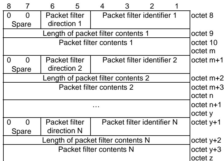
Figure 9.11.4.13.4: Packet filter list when the rule operation is "create new QoS rule", or "modify existing QoS rule and add packet filters" or "modify existing QoS rule and replace all packet filters"
