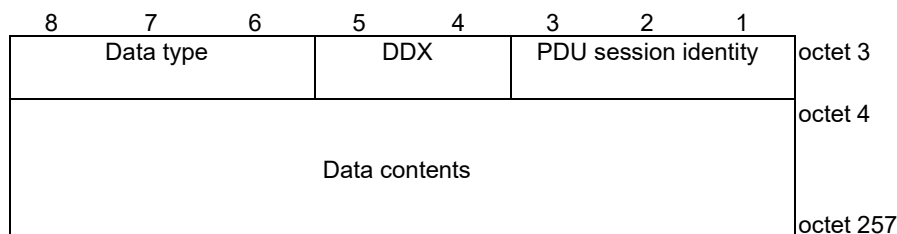
Figure 9.11.3.18B.2: ClIoT small data container contents for Data type "Control plane user data"
