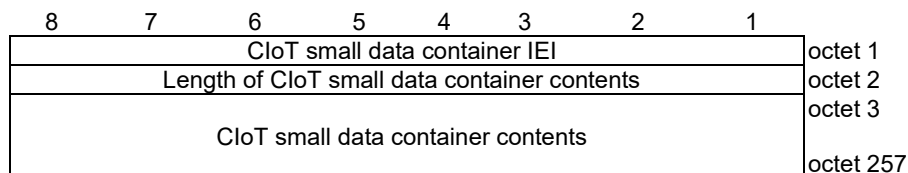
Figure 9.11.3.18B.1: ClIoT small data container information element
