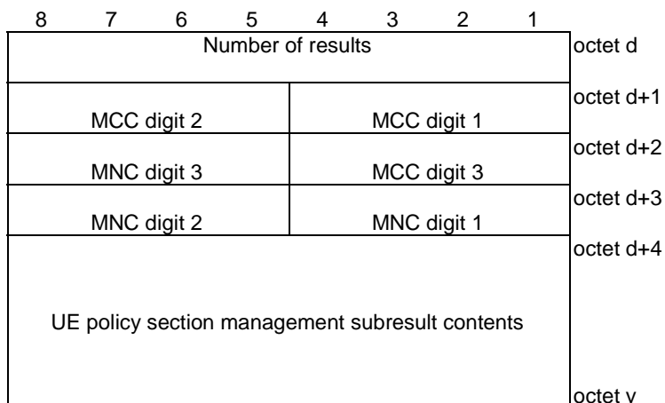
Figure D.6.3.3: UE policy section management subresult
