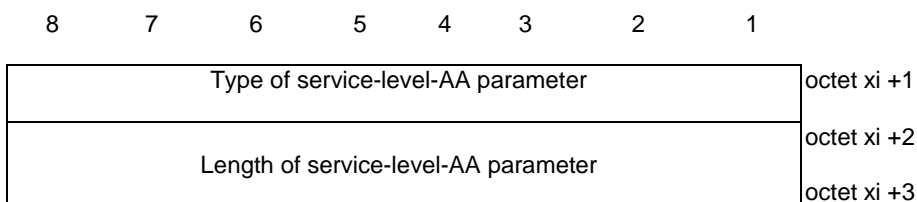
Figure 9.11.2.10.4: Service-level-AA parameter (when the type of service-level-AA parameter field contains an IEI of a type 6 information element as specified in 3GPP TS 24.007 [11])
