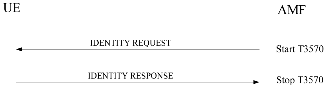
Figure 5.4.3.2.1: Identification procedure
