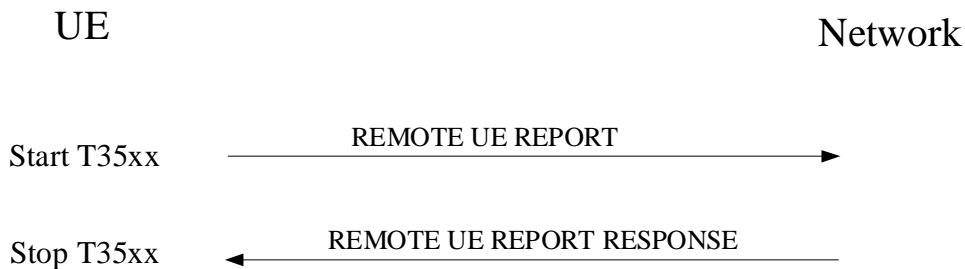
Figure 6.6.2.1: Remote UE report procedure
