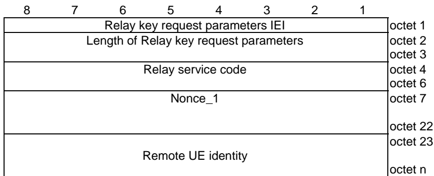
Figure 9.11.3.89.1: Relay key request parameters information element
