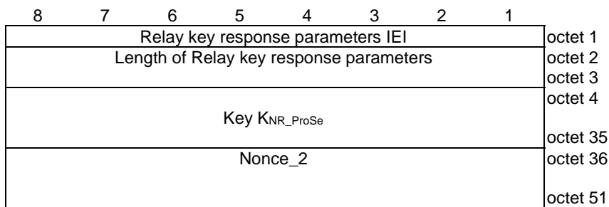
Figure 9.11.3.90.1: Relay key response parameters information element
