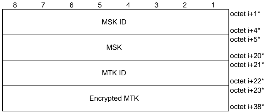
Figure 9.11.4.31.12: MBS security container
