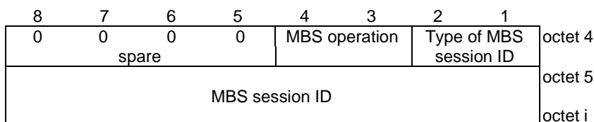
Figure 9.11.4.30.2: MBS session information
