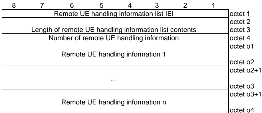
Figure 9.11.4.35.1: Remote UE handling information list information element
