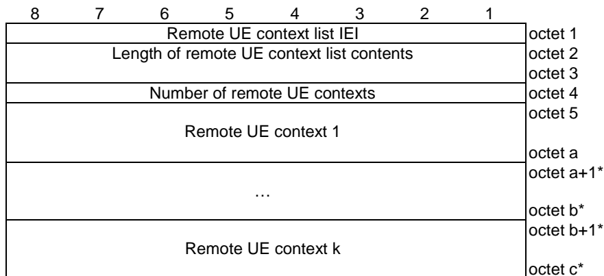
Figure 9.11.4.29.1: Remote UE context list
