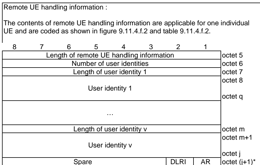
Figure 9.11.4.35.2: Remote UE handling information
