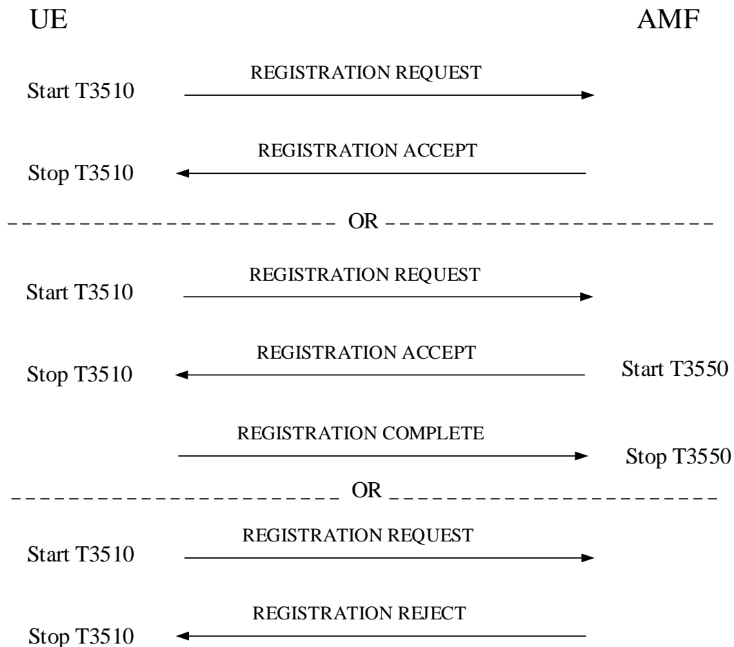
Figure 5.5.1.3.2.1: Registration procedure for mobility and periodic registration update
