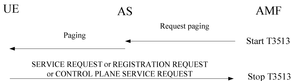
Figure 5.6.2.2.1.1: Paging procedure
