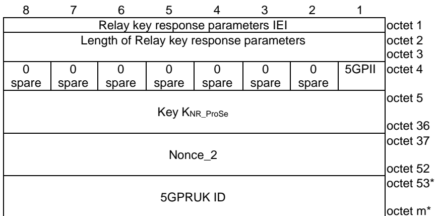
Figure 9.11.3.90.1: Relay key response parameters information element
