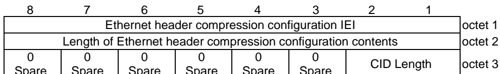
Figure 9.11.4.28.1: Ethernet header compression configuration information element
