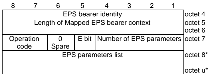
Figure 9.11.4.8.2: Mapped EPS bearer context
