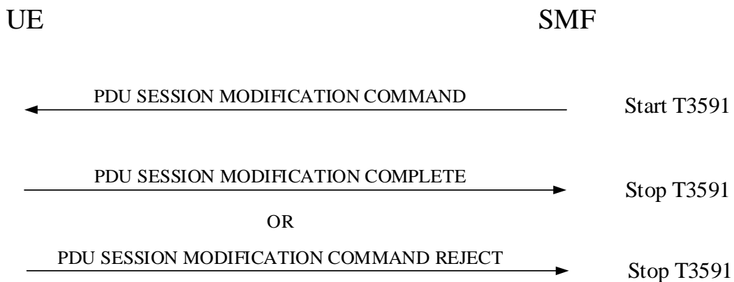
Figure 6.3.2.2.1: Network-requested PDU session modification procedure
