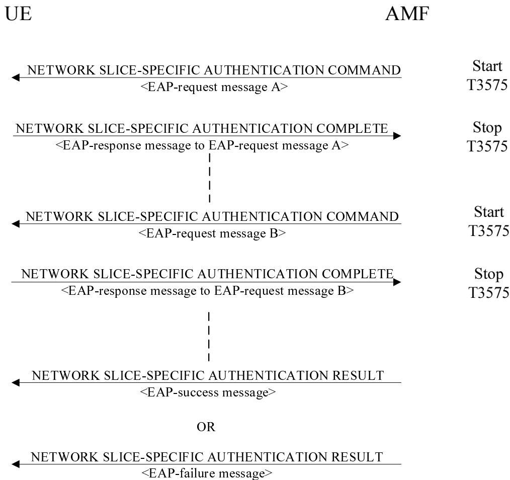
Figure 5.4.7.1.1: Network slice-specific authentication and authorization procedure
