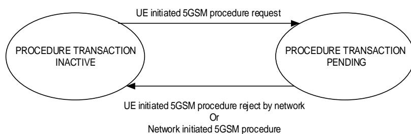
Figure 6.1.3.2.8.1: The procedure transaction states in the UE (overview)
