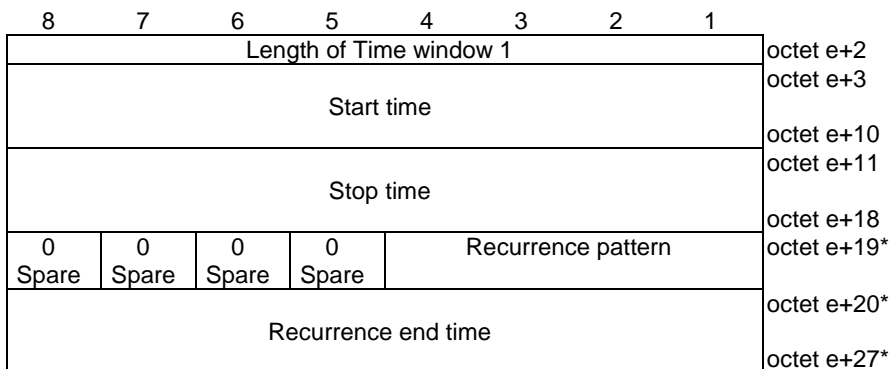
Figure 9.11.3.101.4: Time window 1
