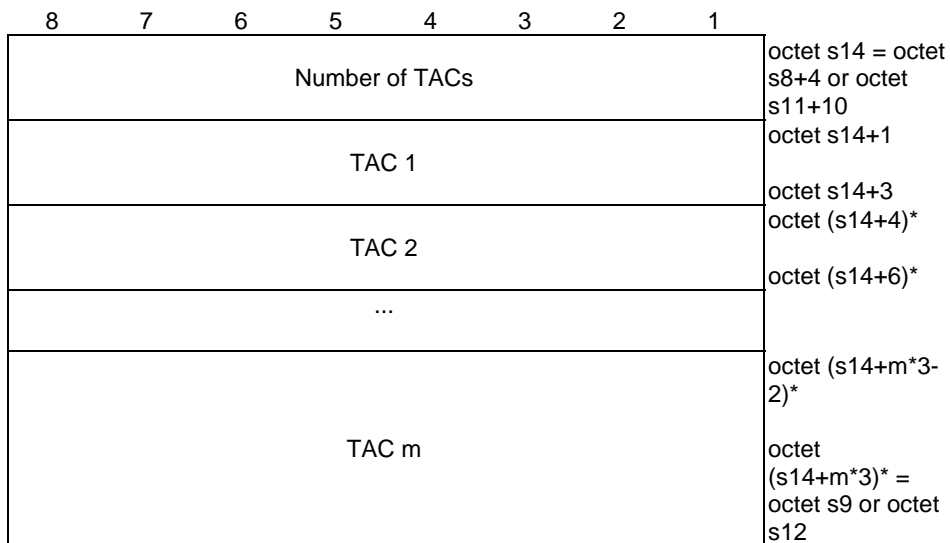
Figure 9.11.3.51.11F: TAC list
