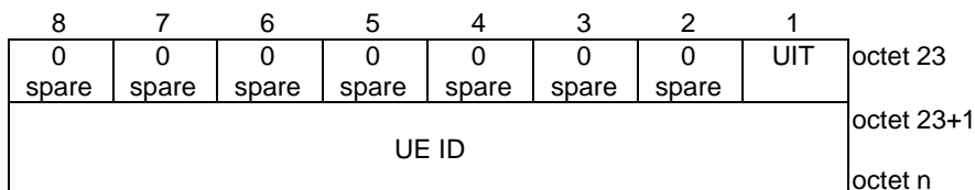
Figure 9.11.3.89.2: UE identity
