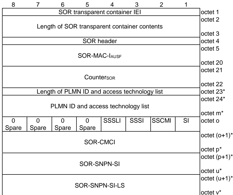
Figure 9.11.3.51.2A: SOR transparent container information element for list type with value "1", SOR data type with value "0", additional parameters with value "1"
