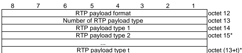
Figure 9.11.4.39.4: RTP payload information
