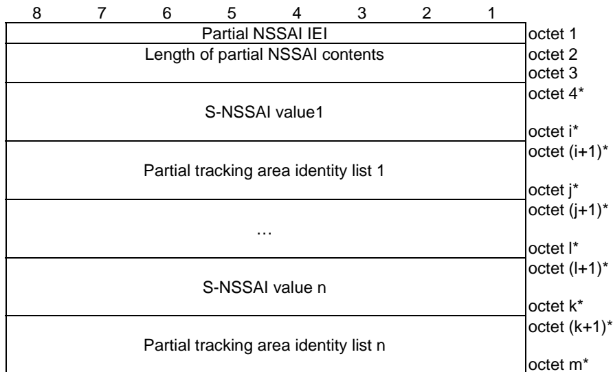
Figure 9.11.3.103.1: Partial NSSAI information element
