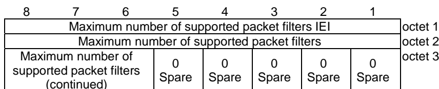
Figure 9.11.4.9.1: Maximum number of supported packet filters information element
