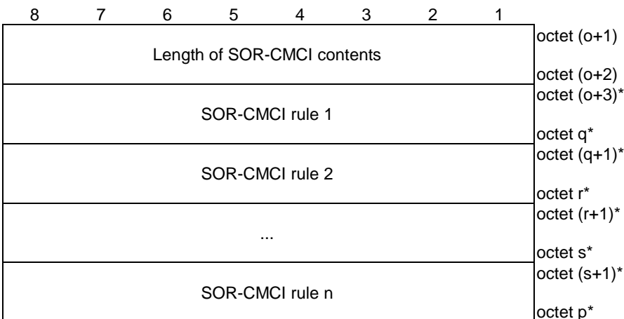
Figure 9.11.3.51.7: SOR-CMCI
