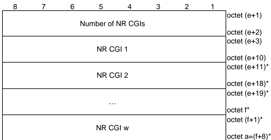
Figure 9.11.3.100.3: NS-AoS
