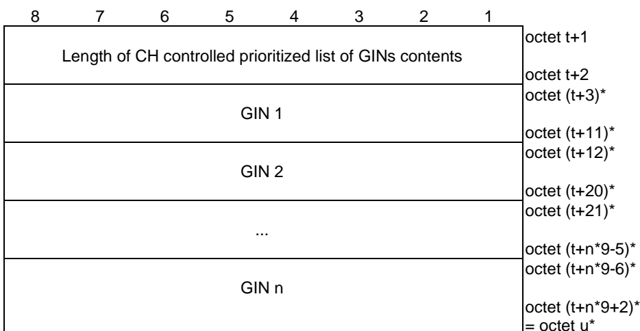
Figure 9.11.3.51.12: CH controlled prioritized list of GINs
