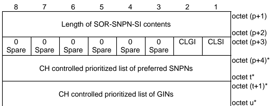
Figure 9.11.3.51.9: SOR-SNPN-SI
