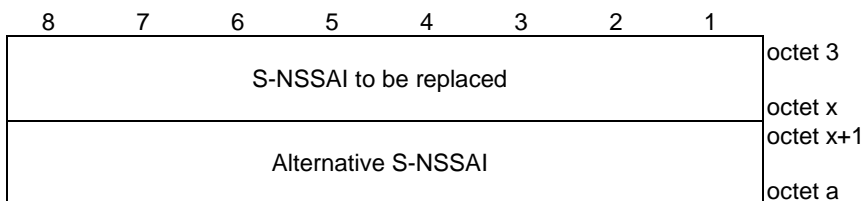
Figure 9.11.3.97.2: Entry
