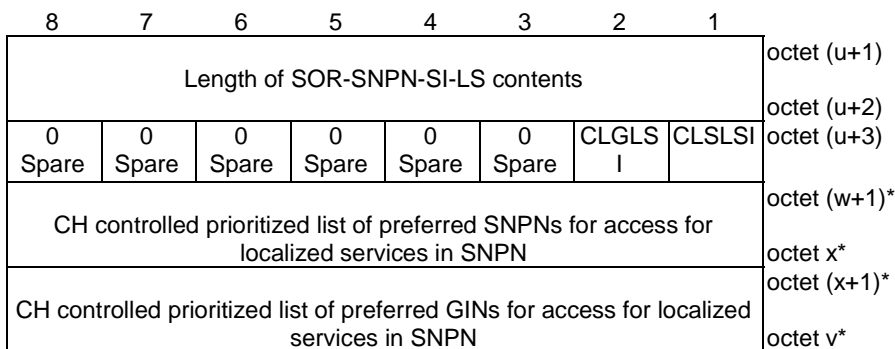
Figure 9.11.3.51.9A: SOR-SNPN-SI-LS
