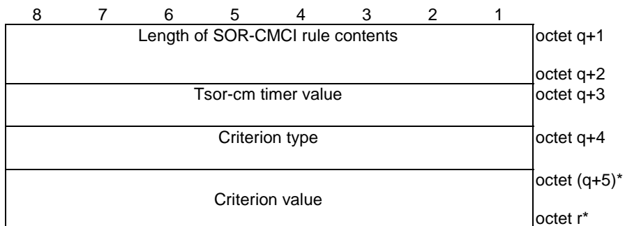
Figure 9.11.3.51.8: SOR-CMCI rule
