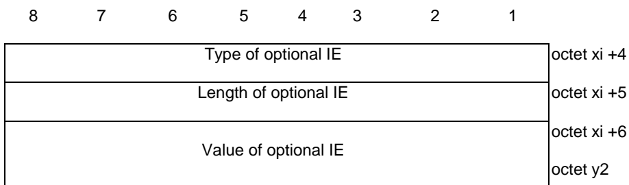
Figure 9.11.3.39.4: Optional IE
