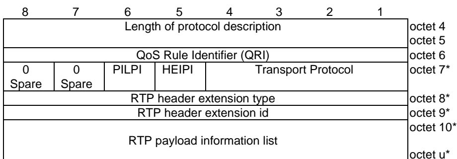
Figure 9.11.4.39.2: Protocol description
