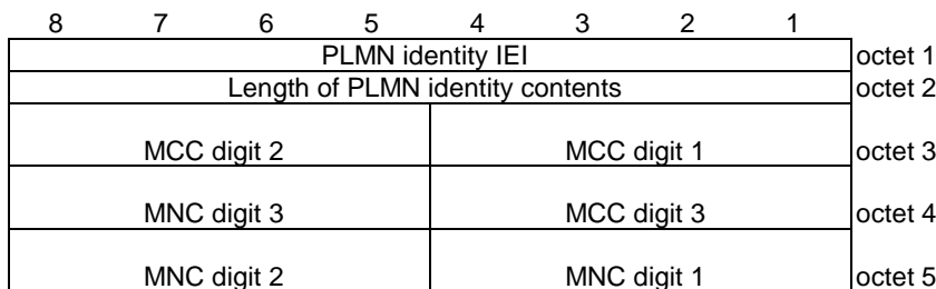
Figure 9.11.3.85.1: PLMN identity information element
