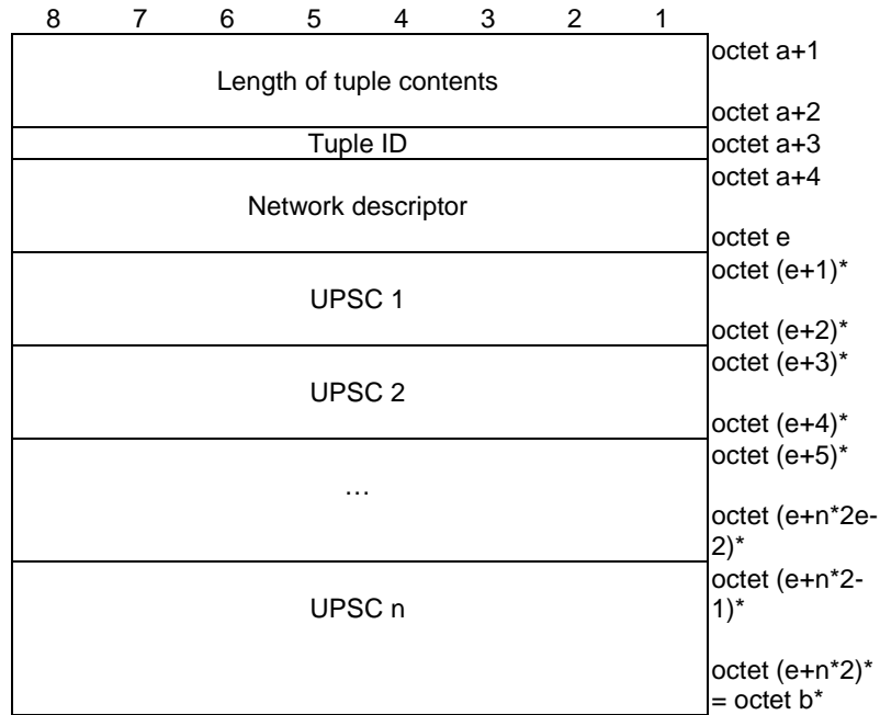
Figure D.6.8.2: Tuple
