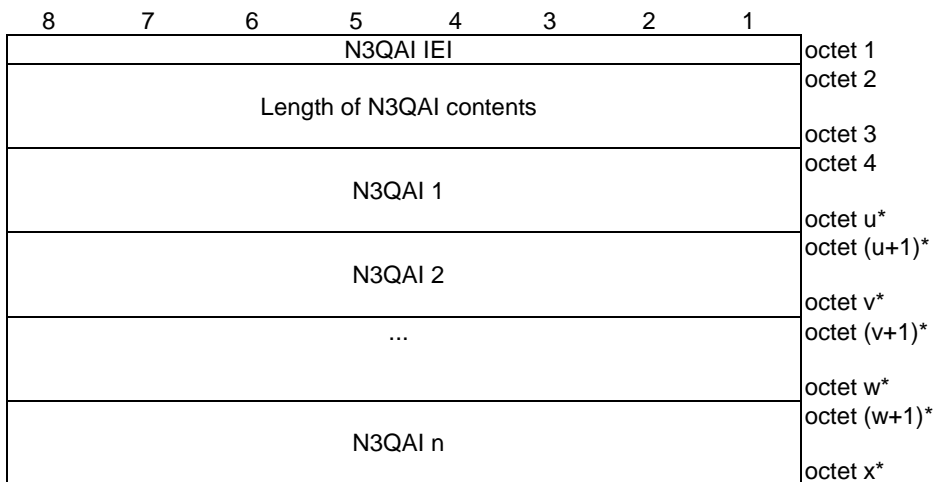
Figure 9.11.4.36.1: N3QAI information element
