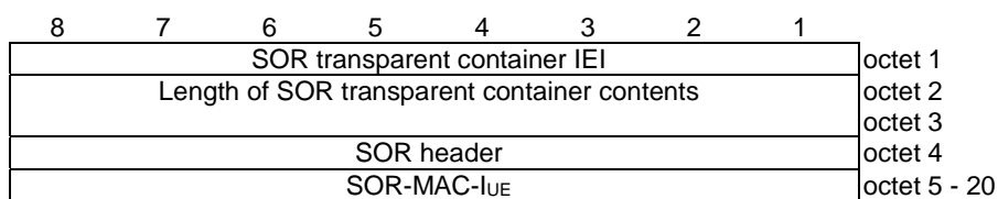
Figure 9.11.3.51.4: SOR transparent container information element for SOR data type with value "1"
