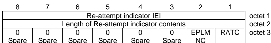
Figure 9.11.4.17.1: Re-attempt indicator
