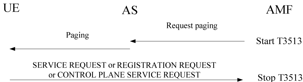
Figure 5.6.2.2.1.1: Paging procedure
