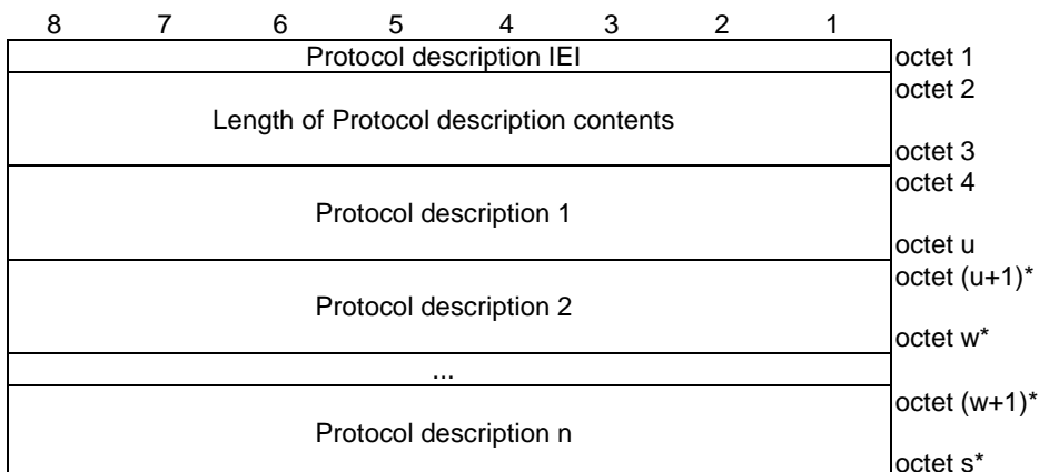
Figure 9.11.4.39.1: Protocol description information element
