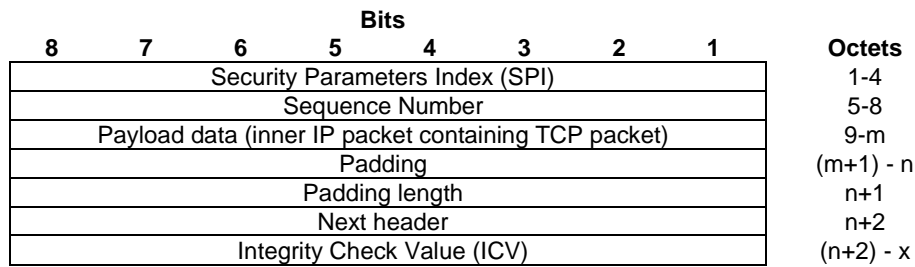
Figure 8.2.2-1: ESP packet format for TCP packet establishing TCP connection
