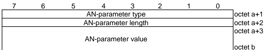
Figure 9.3.2.2.2.1-3: AN-parameter field
