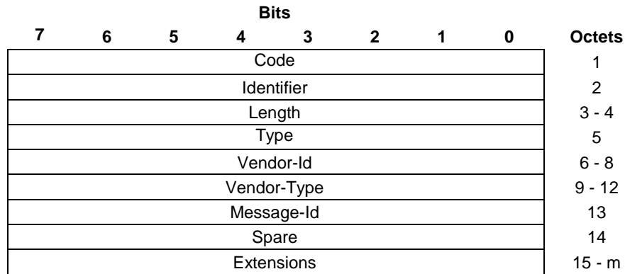
Figure 9.3.2.2.4-1: EAP-Request/5G-Stop message
