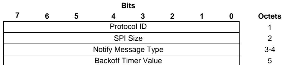
Figure 9.3.1.7-1: N3GPP_BACKOFF_TIMER Notify payload format
