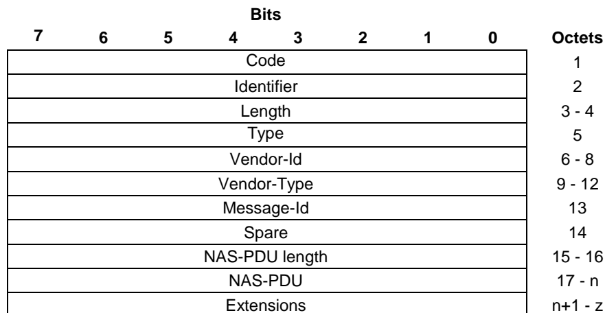
Figure 9.3.2.2.3-1: EAP-Request/5G-NAS message
