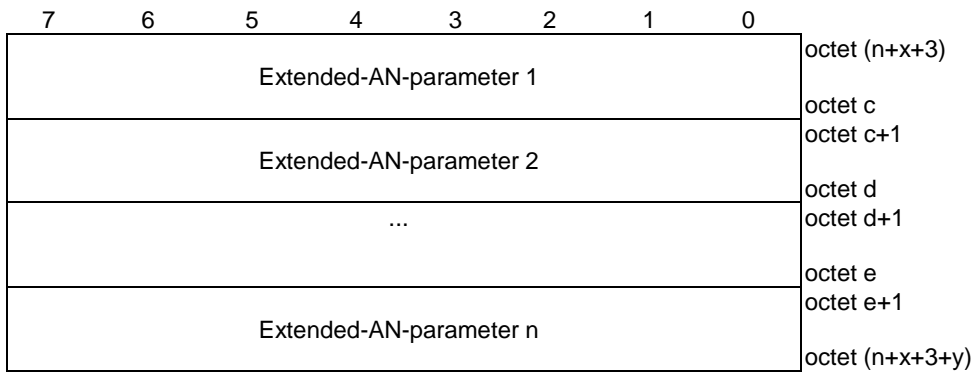
Figure 9.3.2.2.2-4: Extended-AN-parameters field
