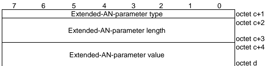
Figure 9.3.2.2.2-5: Extended-AN-parameter field
