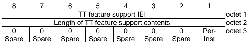
Figure 9.13.1: TT feature support information element
