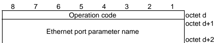
Figure 9.2.4: Operation for operation code set to "00000010", "00000100", or "00000101"
