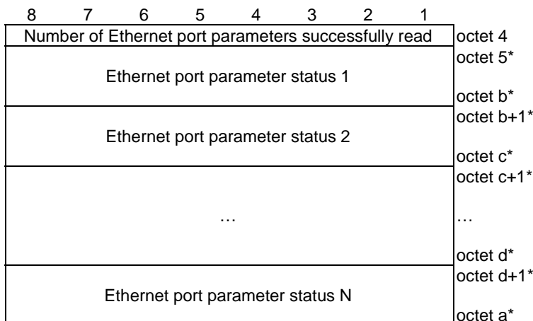
Figure 9.4.2: Ethernet port status contents
