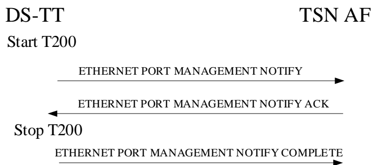
Figure 5.2.2.2.1: DS-TT-initiated Ethernet port management procedure
