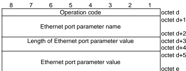
Figure 9.2.5: Operation for operation code set to "00000011"
