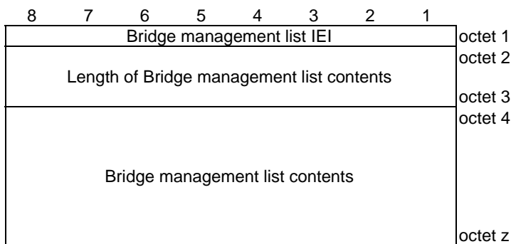
Figure 9.5B.1: Bridge management list information element
