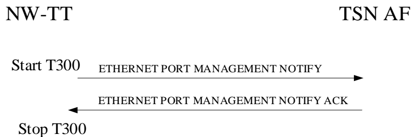
Figure 6.2.2.2.1: NW-TT-initiated Ethernet port management procedure
