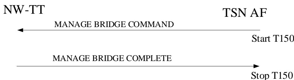
Figure 6.3.1.2.1: TSN AF-requested Bridge management procedure
