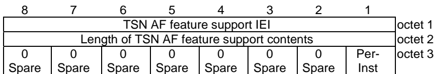
Figure 9.12.1: TSN AF feature support information element
