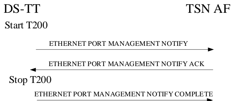
Figure 5.2.2.2.1: DS-TT-initiated Ethernet port management procedure
