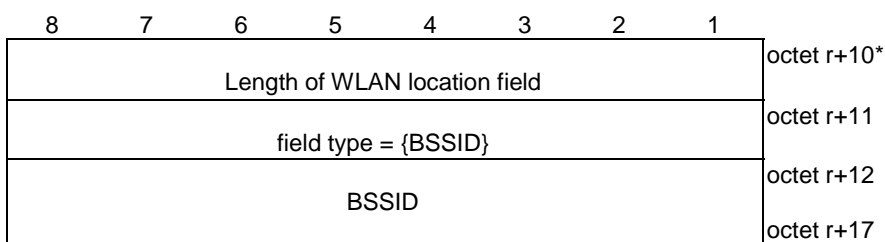
Figure 5.3.2.14c: WLAN location field {field type = BSSID}
