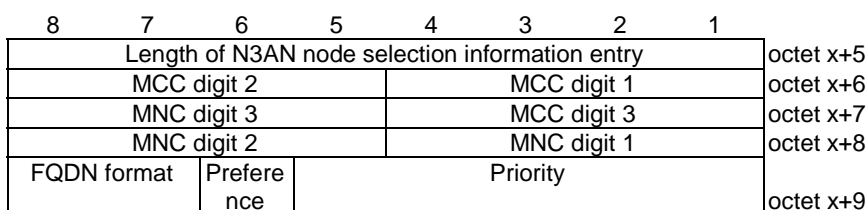
Figure 5.3.3.2.2: N3AN node selection information entry
