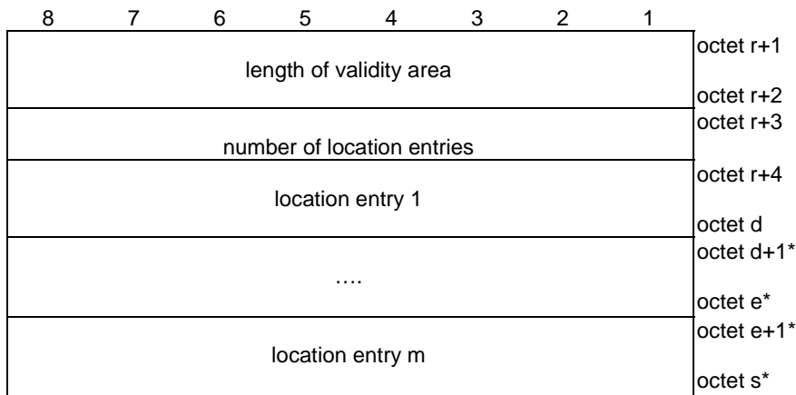
Figure 5.3.2.5: Validity area
