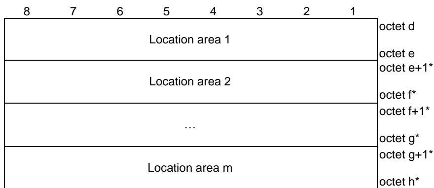
Figure 5.2.5: Location criteria
