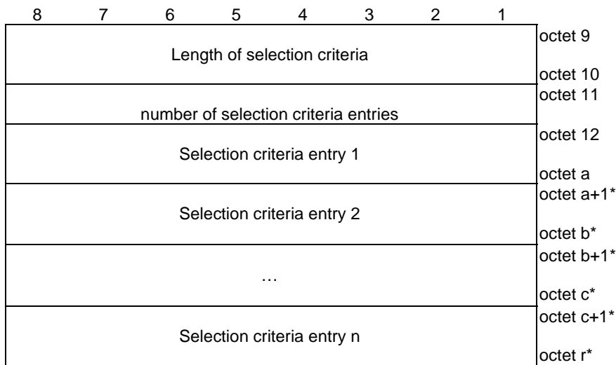
Figure 5.3.2.4: Selection criteria
