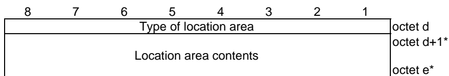
Figure 5.2.6: Location area
