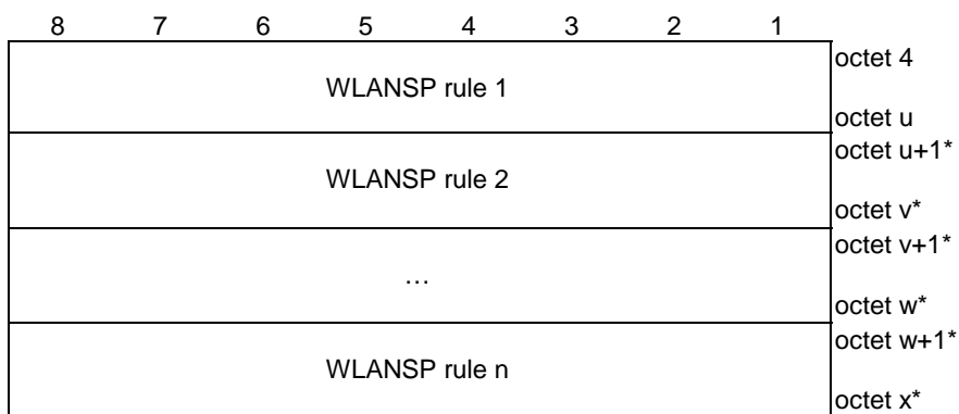
Figure 5.3.2.2: WLANSP contents
