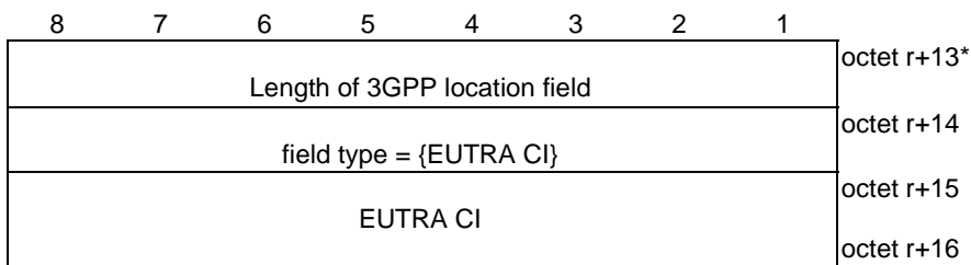
Figure 5.3.2.13: 3GPP location field {field type = EUTRA CI}
