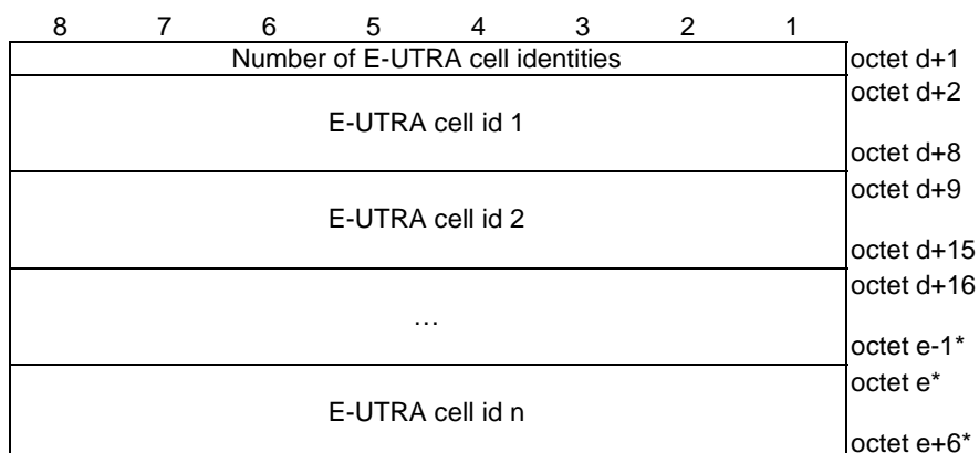
Figure 5.2.7: Location area contents {Type of location area = E-UTRA cell identities list}
