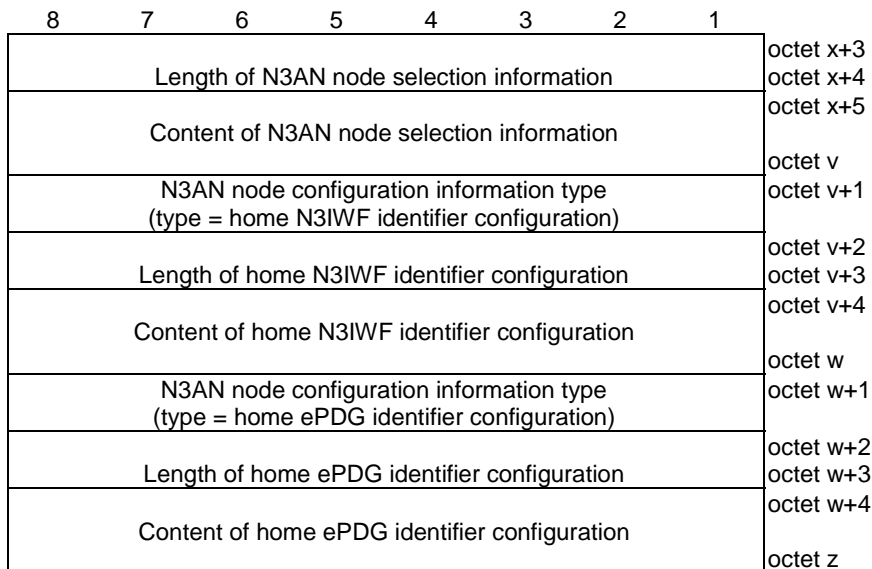
Figure 5.3.3.1.2: N3AN node configuration information contents
