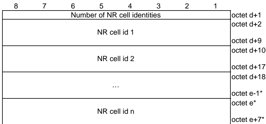
Figure 5.2.8: Location area contents {Type of location area = NR cell identities list}
