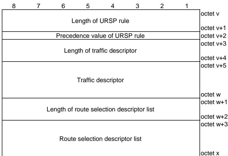
Figure 5.2.2: URSP rule
