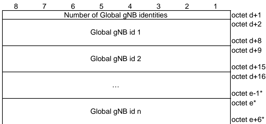
Figure 5.2.9: Location area contents {Type of location area = Global RAN node identities list}
