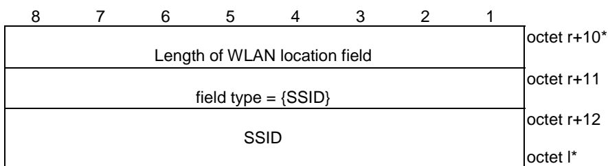
Figure 5.3.2.14b: WLAN location field {field type = SSID}
