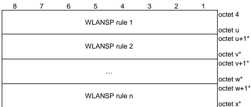
Figure 5.3.2.2: WLANSP contents
