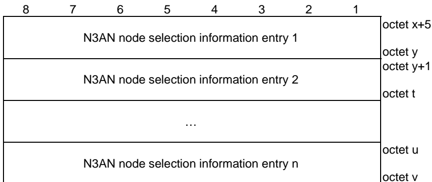
Figure 5.3.3.2.1: Content of N3AN node selection information
