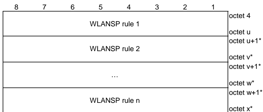
Figure 5.3.2.2: WLANSF contents
