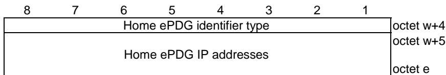
Figure 5.3.3.4.2: Home ePDG identifier entry (Home ePDG identifier type = "IPv4", "IPv6" or "IPv4v6")
