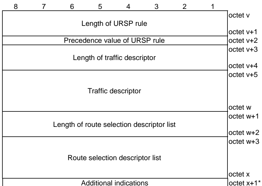
Figure 5.2.2: URSP rule
