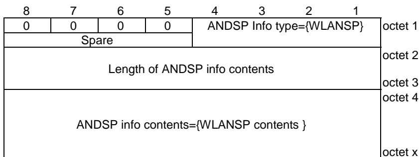
Figure 5.3.2.1: ANDSP Info type = {WLANSP}
