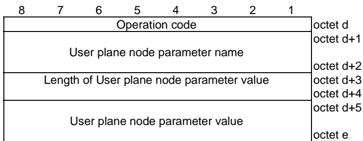
Figure 9.5B.5: Operation for operation code set to "0000011", "0000110", "0000111", "0000100" and "0000101"
