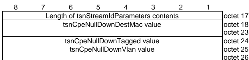
Figure 9.8.3: tsnStreamIdParameters for tsnStreamIdIdentificationType = 00-80-C2 01
