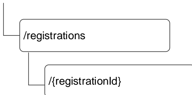
Figure 6.2.2.1-1: Resource URI structure of the Eees_EECRegistration API
