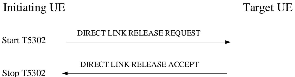
Figure 6.1.2.4.2.1: A2X PC5 unicast link release procedure
