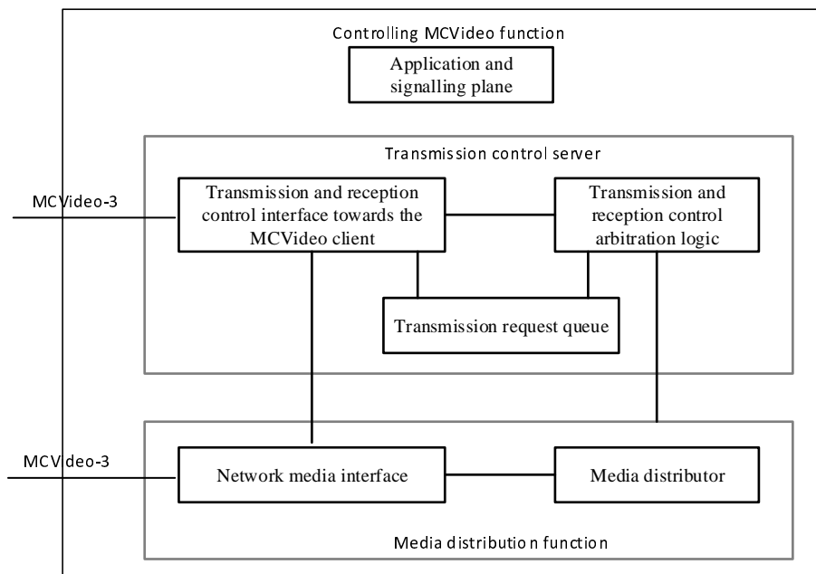
Figure 4.2.1-1: Internal structure of transmission control in the controlling MCVideo function
