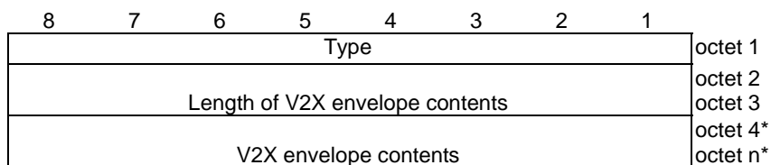
Figure 9.2.1.1: General format of V2X envelope
