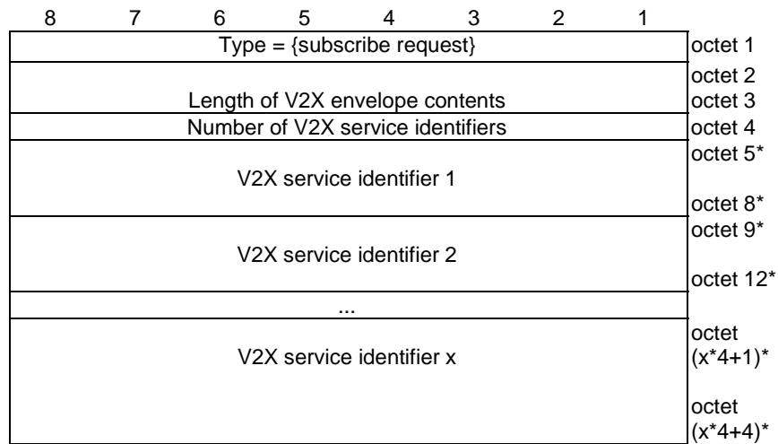
Figure 9.2.1.4: Format of V2X envelope with subscribe request
