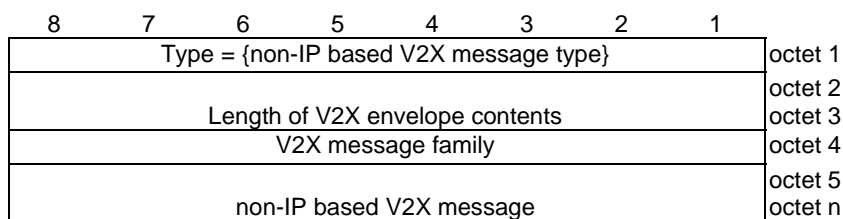
Figure 9.2.1.3: Format of V2X envelope for non-IP based V2X message
