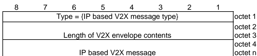
Figure 9.2.1.2: Format of V2X envelope for IP based V2X message
