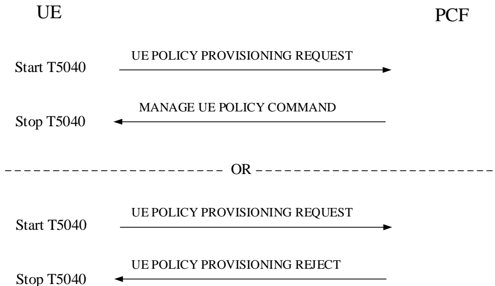
Figure 5.3.2.2.1: UE-requested V2X policy provisioning procedure
