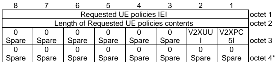
Figure 8.3.2.1: Requested UE policies information element
