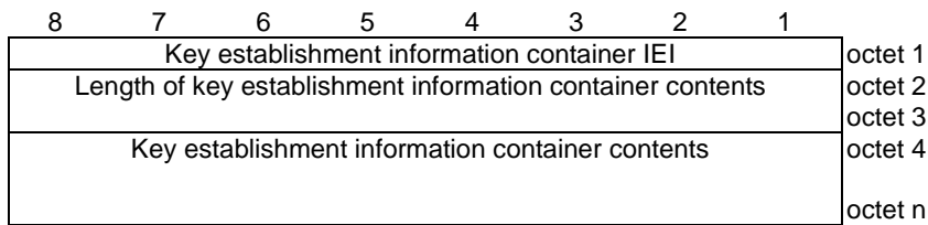
Figure 8.4.a.1: Key establishment information container information element
