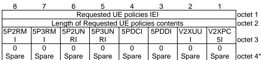
Figure 8.3.2.1: Requested UE policies information element
