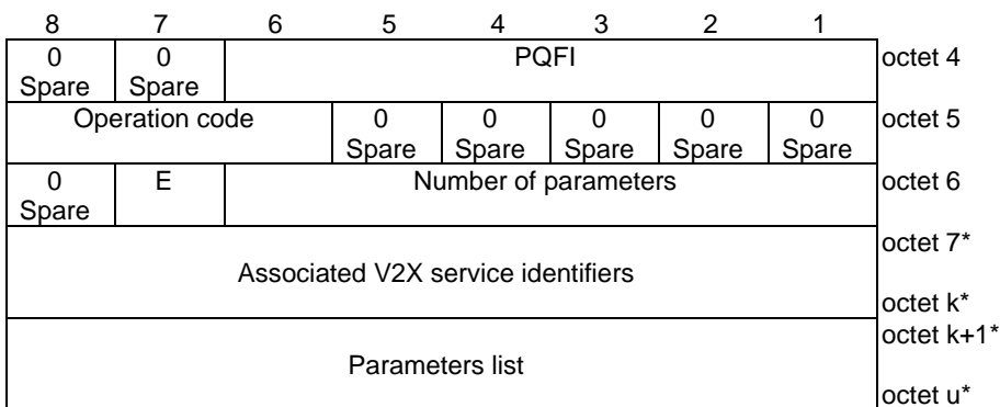
Figure 8.4.5.2: PC5 QoS flow description
