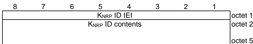
Figure 8.4.17.1: K_{\text{NRP}} ID information element
