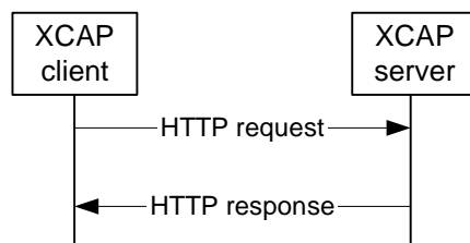
Figure 3: XCAP architecture
