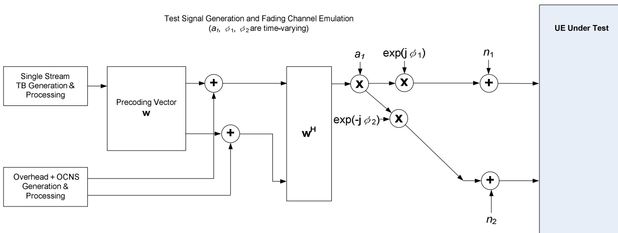
Figure B.4: Test setup under MIMO Single Stream Fading Conditions
