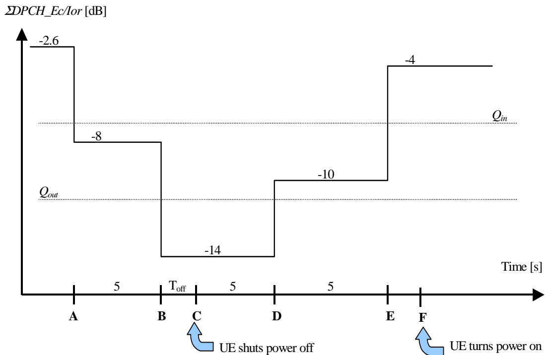
Figure 6.1AA: Test case for out-of-synch handling in the UE - 1.28 Mcps TDD option – continuous transmission
