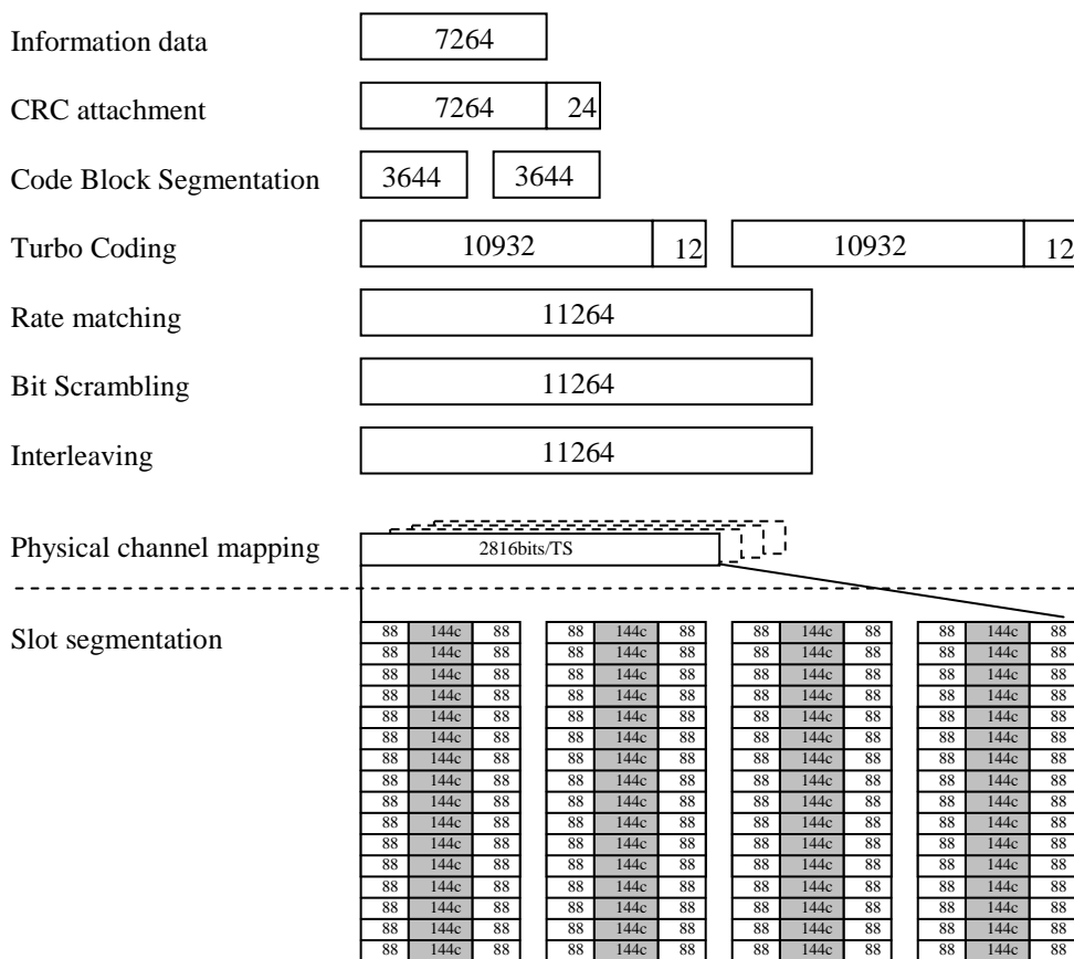
Figure A.26A Reference Measurement Channel for Category 26 (16QAM) - First Stream
