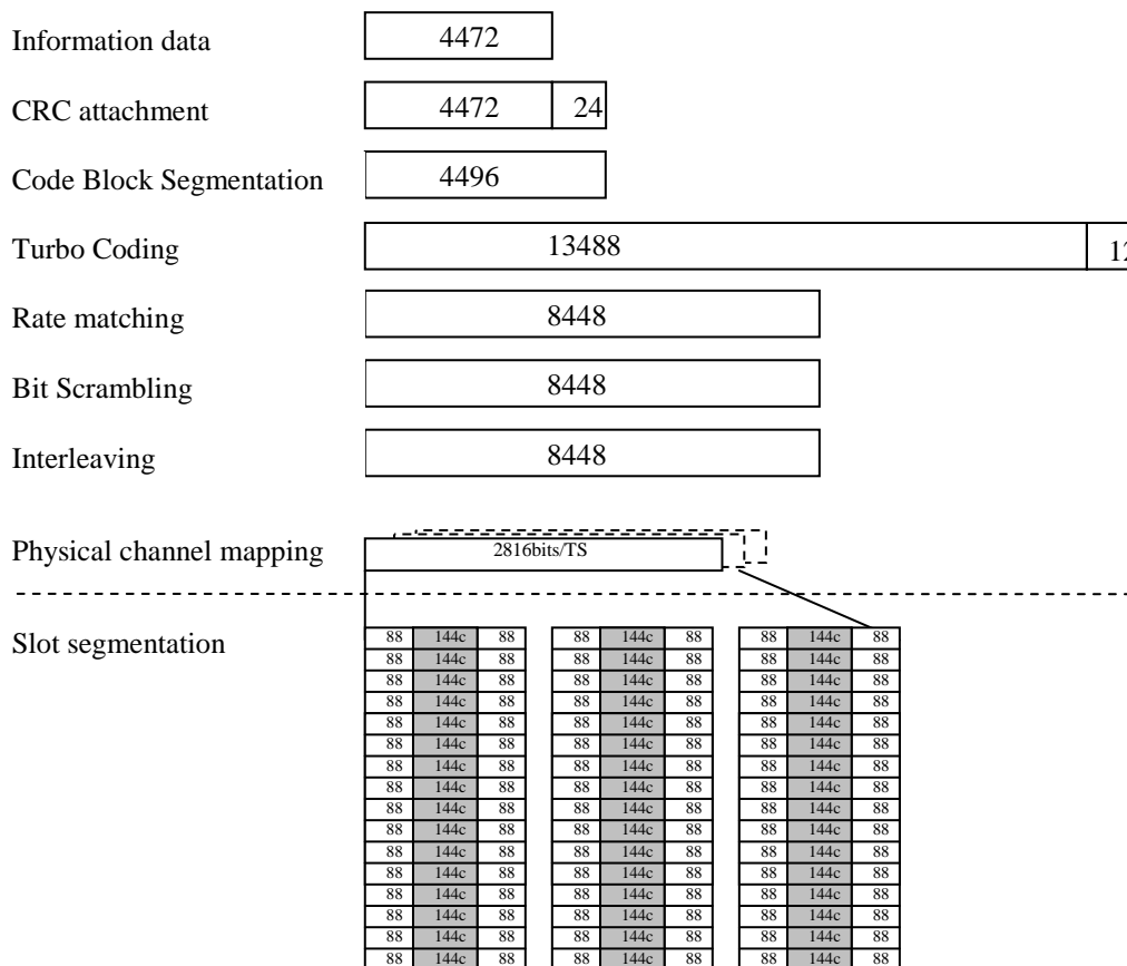
Figure A.23A Reference Measurement Channel for Category 25 (16QAM) - Second Stream
