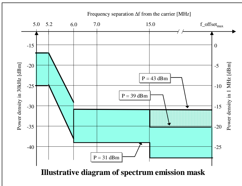
Figure 6.2B: Spectrum emission mask
