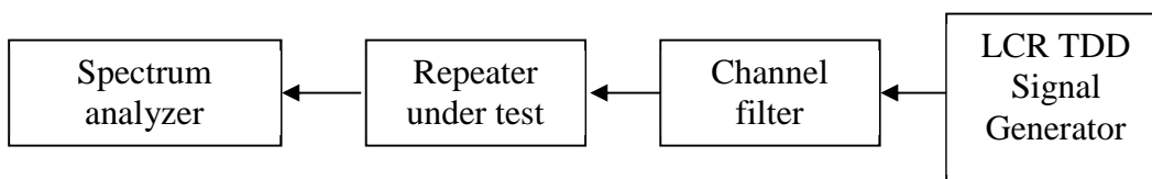
Figure A.4: Measuring system Set-up for unwanted emission: spectrum emission mask.
