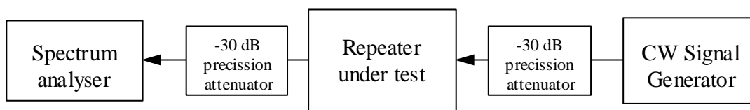
Figure A.3: Measuring system set-up for out of band gain.
