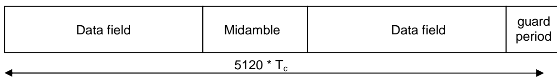
Figure 6.2.1: 7.68Mcps TDD option burst structure
