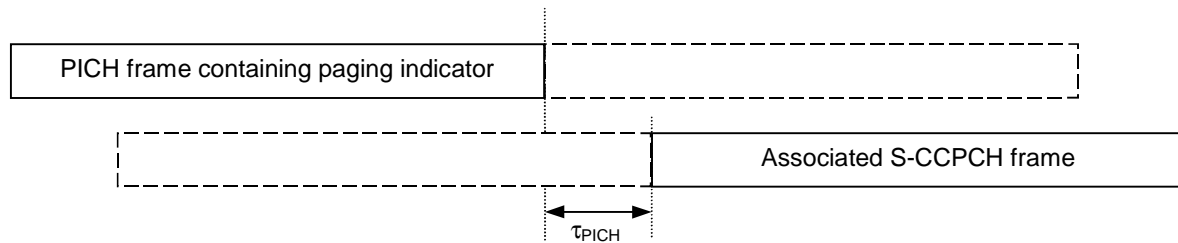
Figure 28: Timing relation between PICH frame and associated S-CCPCH frame
