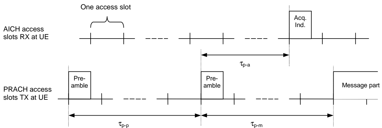
Figure 29: Timing relation between PRACH and AICH as seen at the UE
