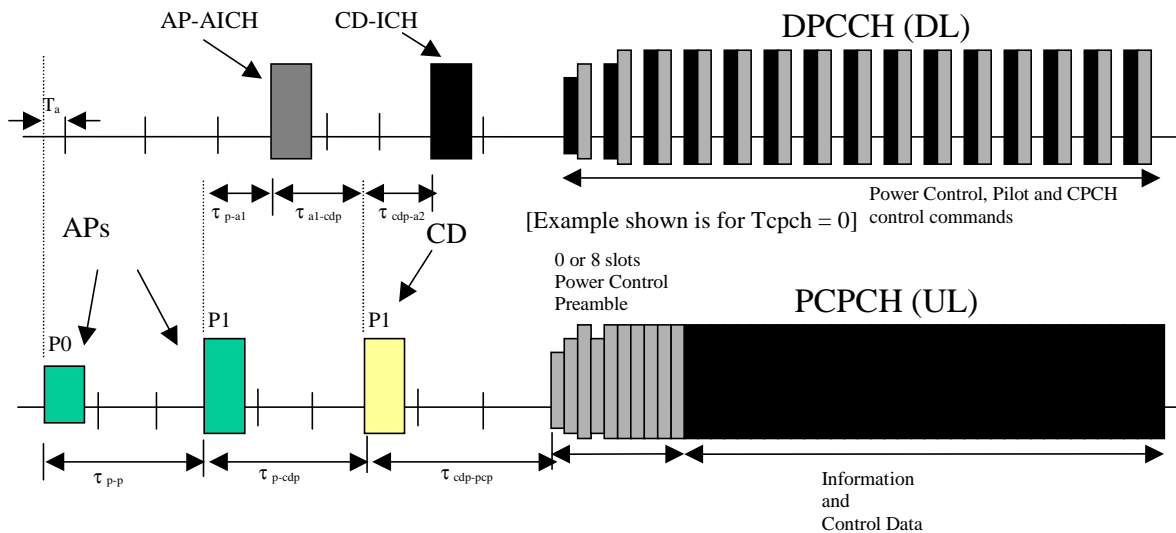
Figure 30: Timing of PCPCH and AICH transmission as seen by the UE, with T_{cpch} = 0
