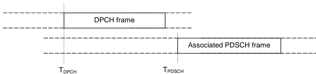
Figure 31: Timing relation between DPCH frame and associated PDSCH frame
