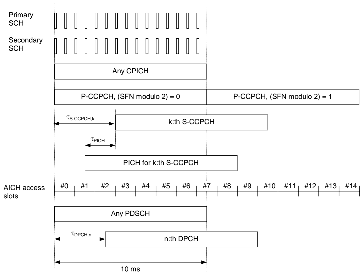
Figure 27: Frame timing and access slot timing of downlink physical channels
