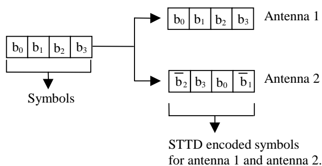
Figure 8: Generic block diagram of the STTD encoder
