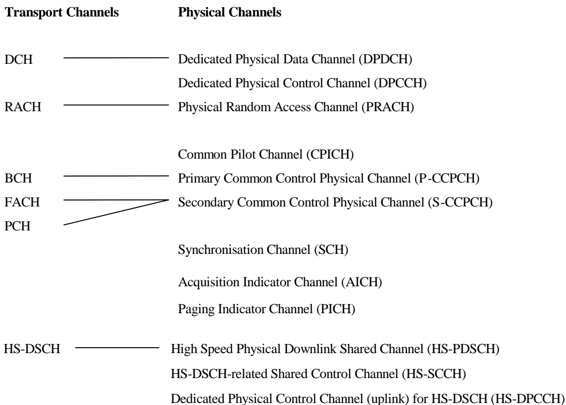
Figure 27: Transport-channel to physical-channel mapping
