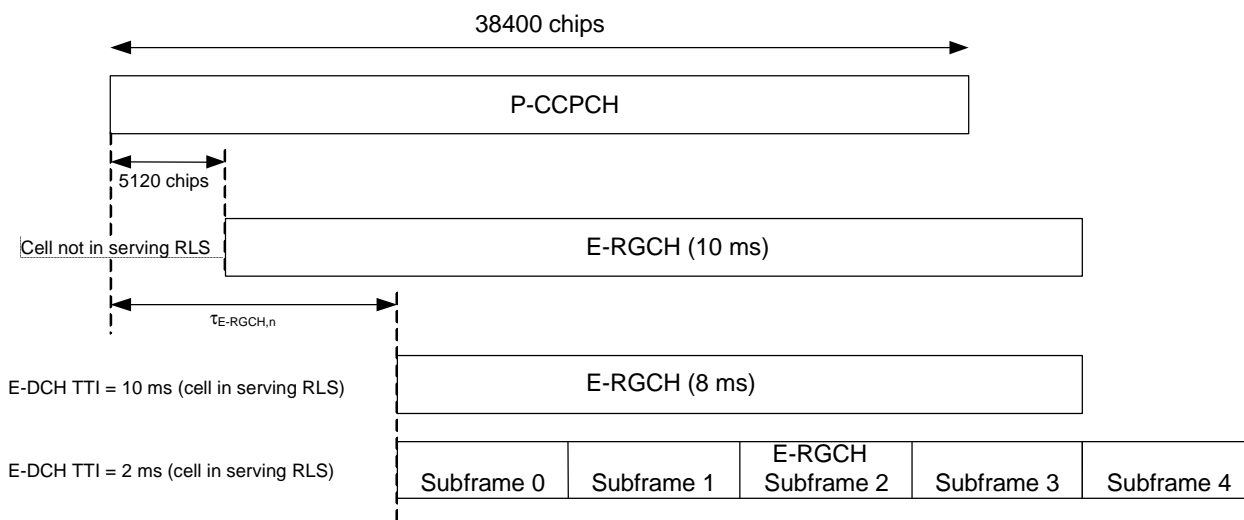
Figure 38: E-RGCH timing
