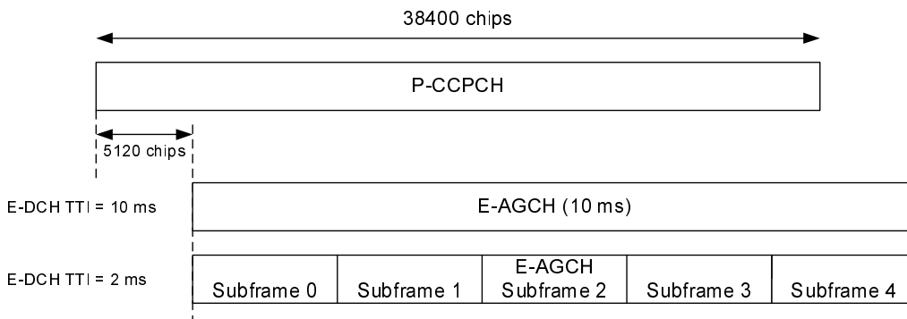
Figure 39: E-AGCH timing
