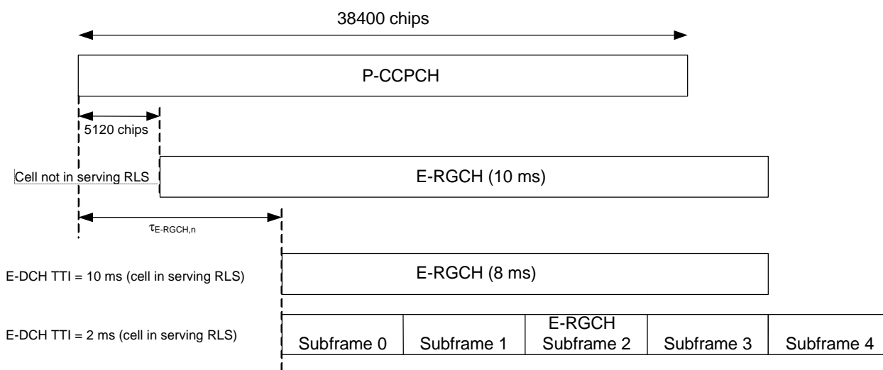
Figure 38: E-RGCH timing
