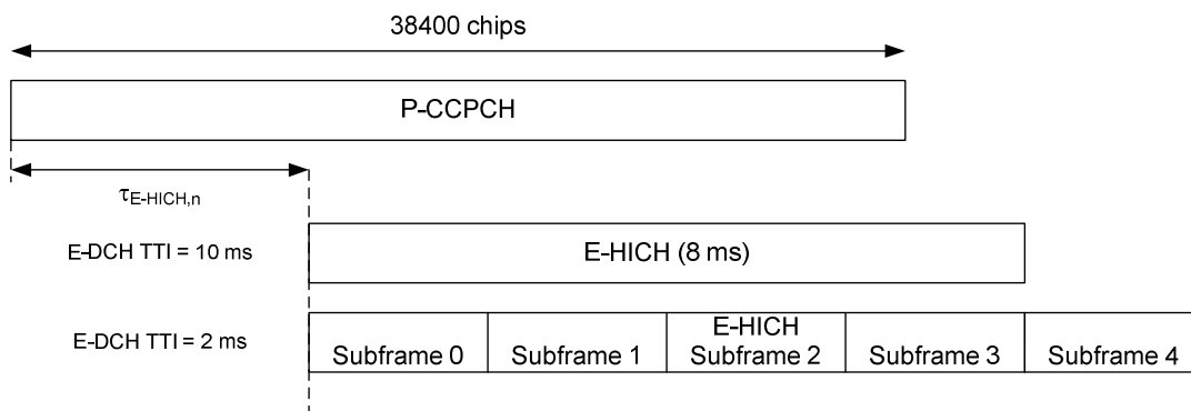
Figure 37: E-HICH timing
